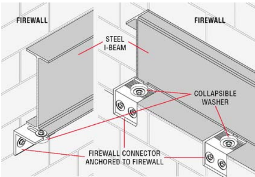
FIG. 2 – Beam Support Detail. For lateral support of the firewall
