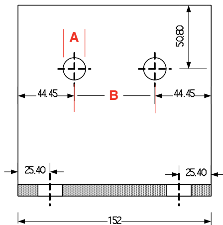
FIG 4 – ANGLE FOR TABLE 1
