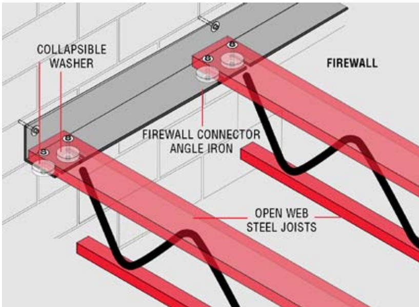
FIG. 1 - Joist Support Detail
